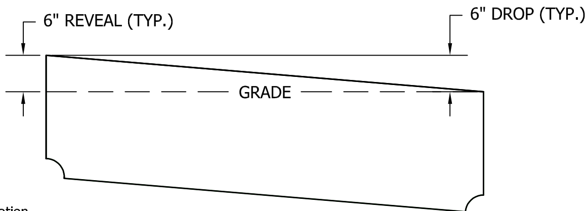
Elevation 3/4" = 1'-0"
