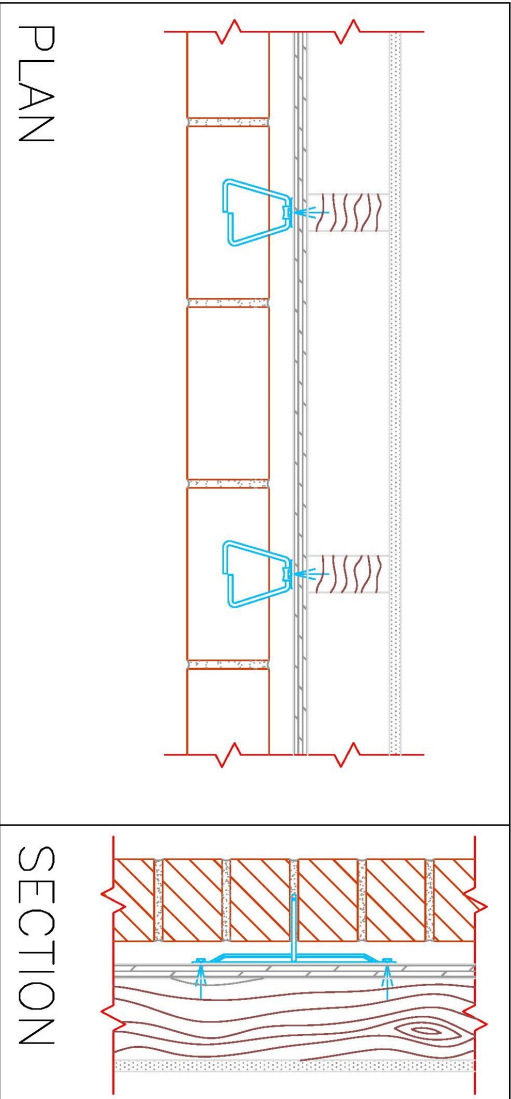
DW-10 Anchor System – Basic System
