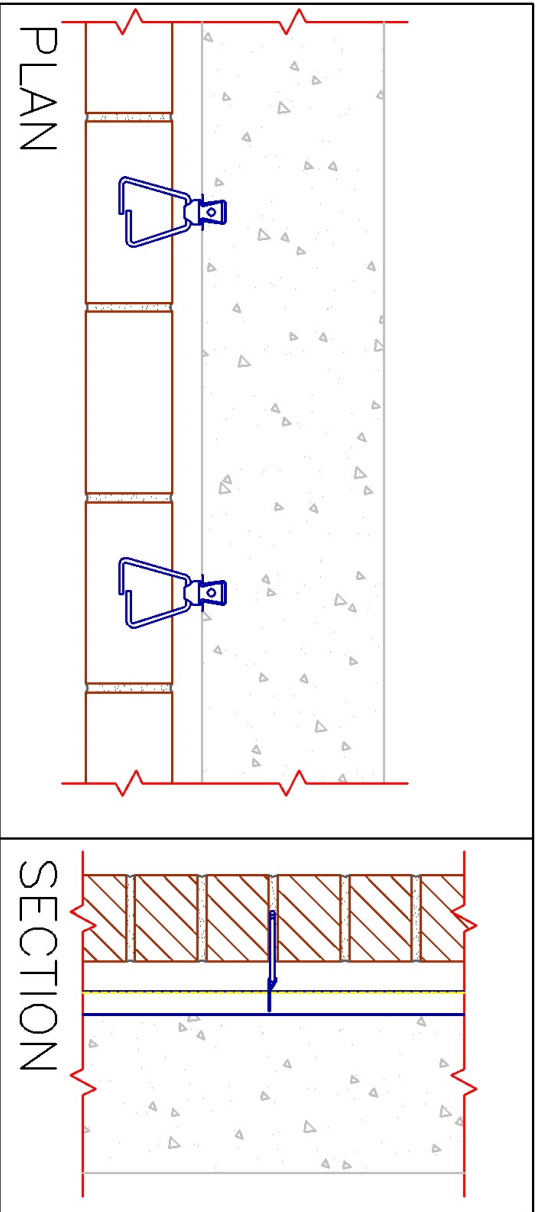
#315 – Flexible Dovetail Tie
